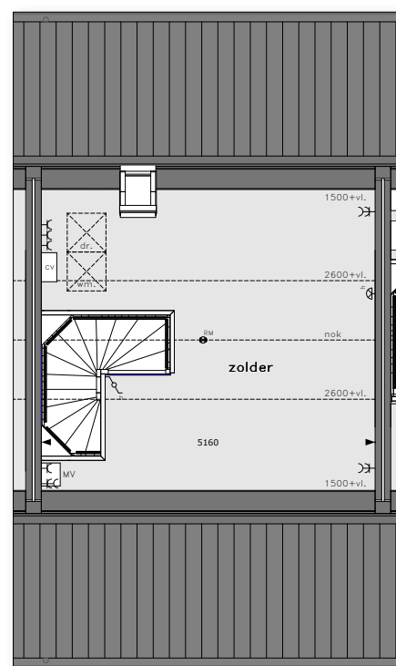
ZOLDER
